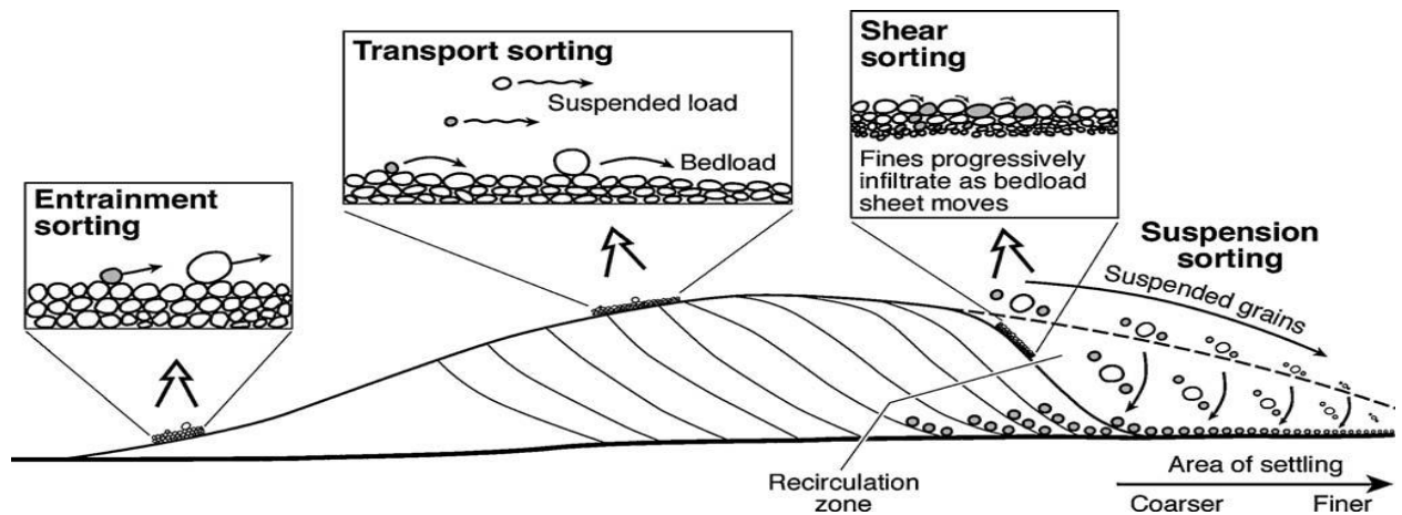
Fig. 5. Distribution and redistribution of heavy mineral concentrations on gravel bar front.
